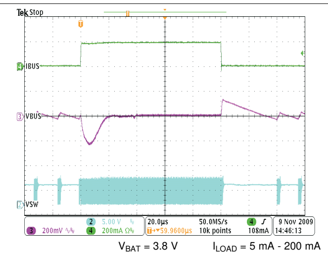
Figure 14. Transient Response
