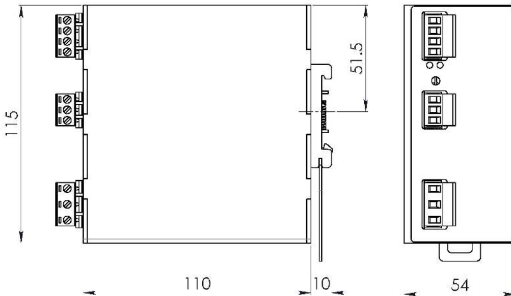
Figure 1. Mechanical Drawing
