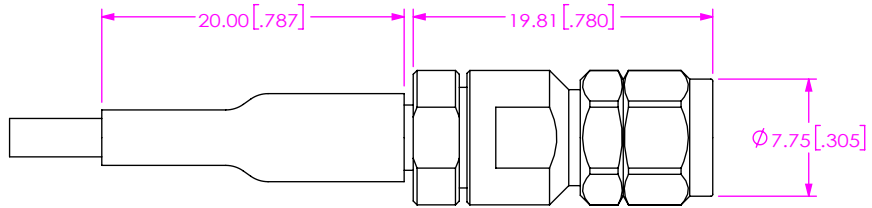
FIG 10 -18SP SHOWN (CABLE CUT FOR CLARITY ONLY)
