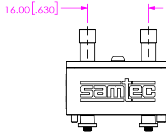
FIG 6 BE70A-S-XXXX-X-2-06-XXXX SHOWN CABLE ASSEMBLIES NOT SHOWN FOR CLARITY
