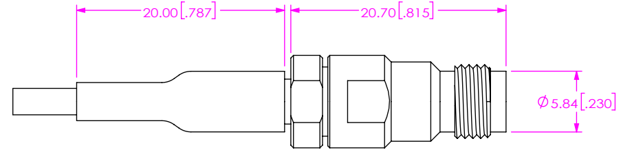
FIG 11 -18SJ SHOWN (CABLE CUT FOR CLARITY ONLY)
