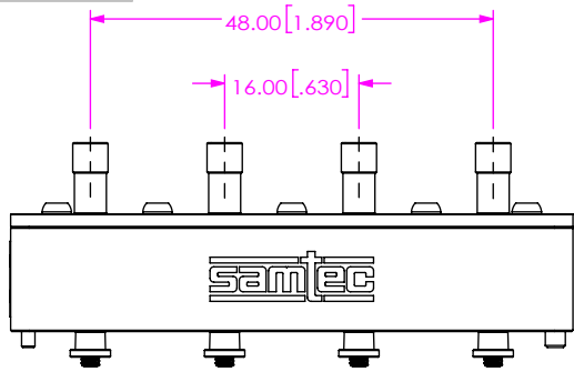
FIG 2 BE70A-S-XXXX-X-2-16-XXXX SHOWN CABLE ASSEMBLIES NOT SHOWN FOR CLARITY
