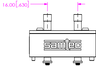
FIG 5 BE70A-S-XXXX-X-2-08-XXXX SHOWN CABLE ASSEMBLIES NOT SHOWN FOR CLARITY
