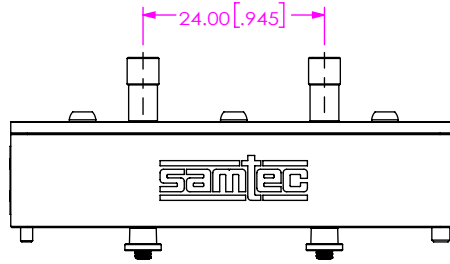
FIG 3 BE70A-S-XXXX-X-2-14-XXXX SHOWN CABLE ASSEMBLIES NOT SHOWN FOR CLARITY
