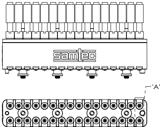
FIG 9 BE70A-M-XXXX-X-2-16-XXXX SHOWN (DIFFERENT AS SHOWN, OTHERWISE SAME AS FIG 2) END 2 NOT SHOWN FOR CLARITY
