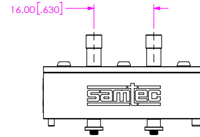
FIG 4 BE70A-S-XXXX-X-2-10-XXXX SHOWN CABLE ASSEMBLIES NOT SHOWN FOR CLARITY
