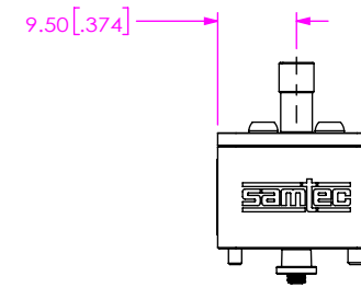
FIG 7 BE70A-S-XXXX-X-2-04-XXXX SHOWN CABLE ASSEMBLIES NOT SHOWN FOR CLARITY
