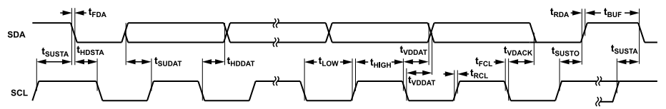
Figure 17. I 2 C Interface Timing Diagram
