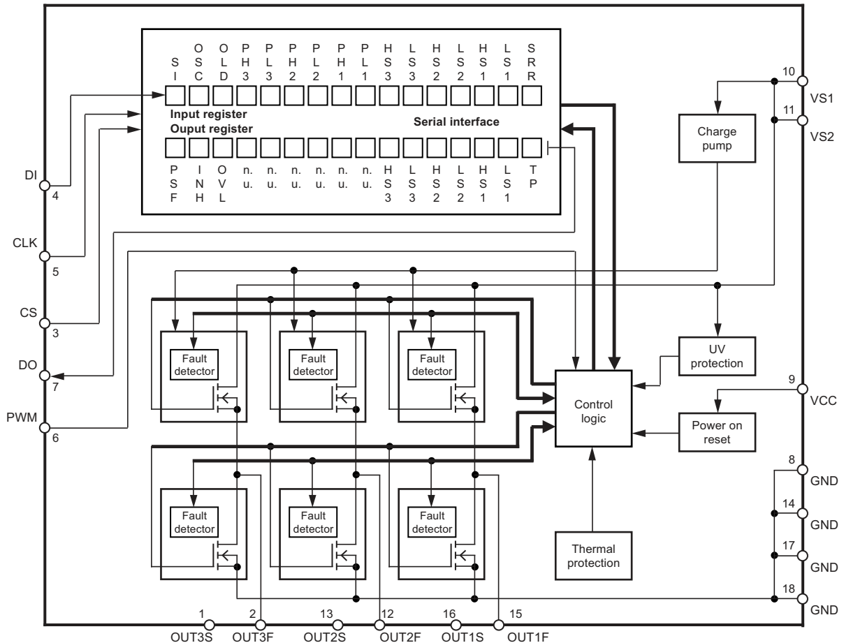
Figure 1-1. Block Diagram
