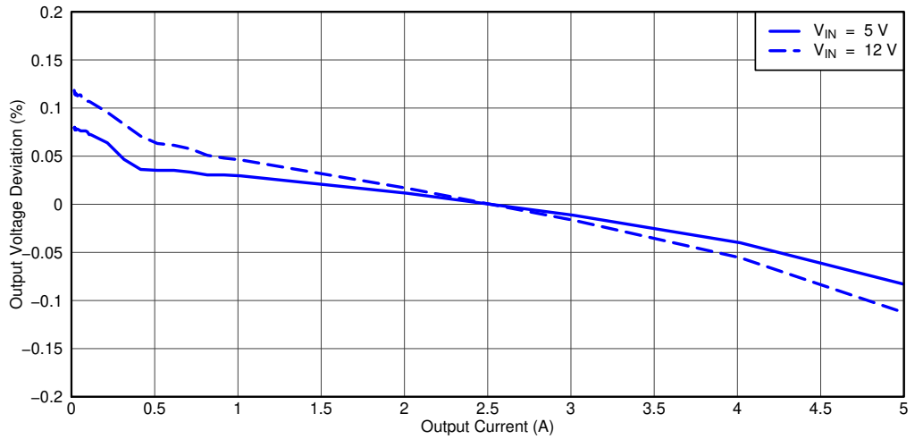
Figure 4-3. TPS54527EVM-052 Load Regulation, V_{IN} = 5\text{ V} and V_{IN} = 12\text{ V}
