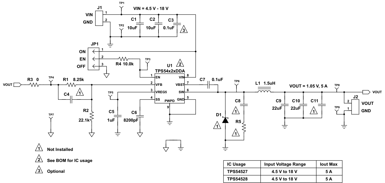
Figure 6-1. TPS54527EVM-052 Schematic Diagram
