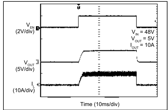
FIGURE 2-54: Enable Turn-On/Turn-Off.
