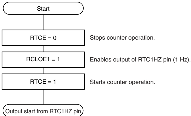
Figure 8-24. 1 Hz Output Setting Procedure
