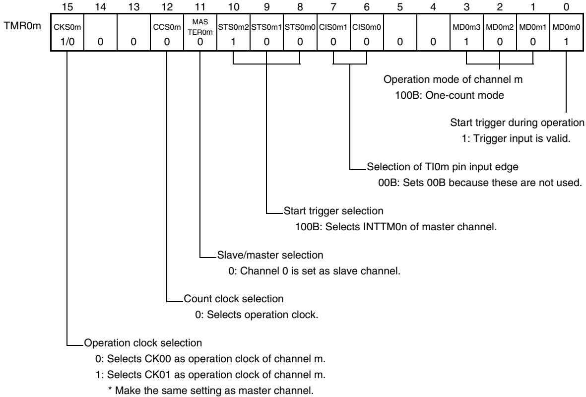
Figure 7-58. Example of Set Contents of Registers When PWM Function (Slave Channel) Is Used
