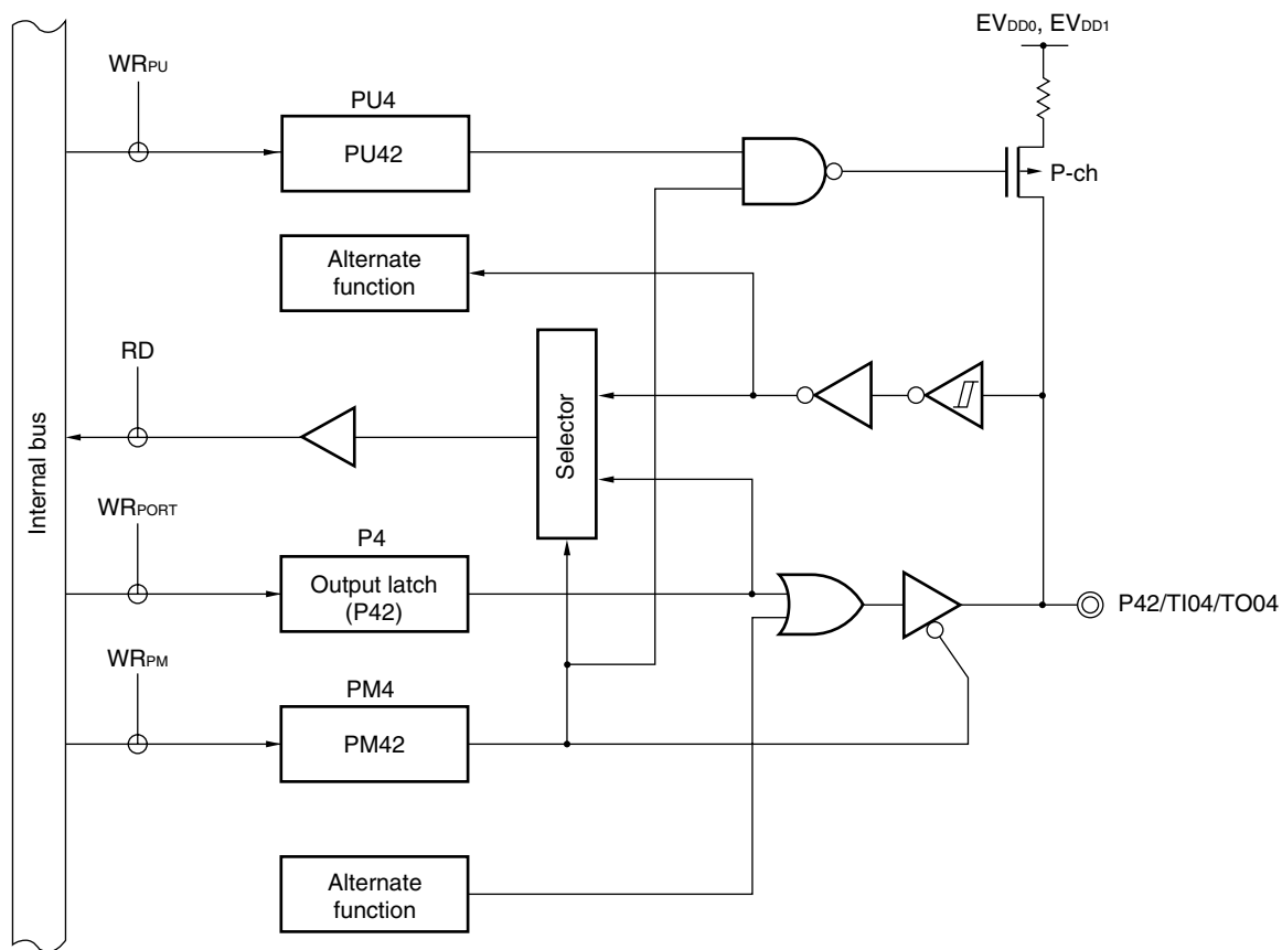
Figure 4-17. Block Diagram of P42
