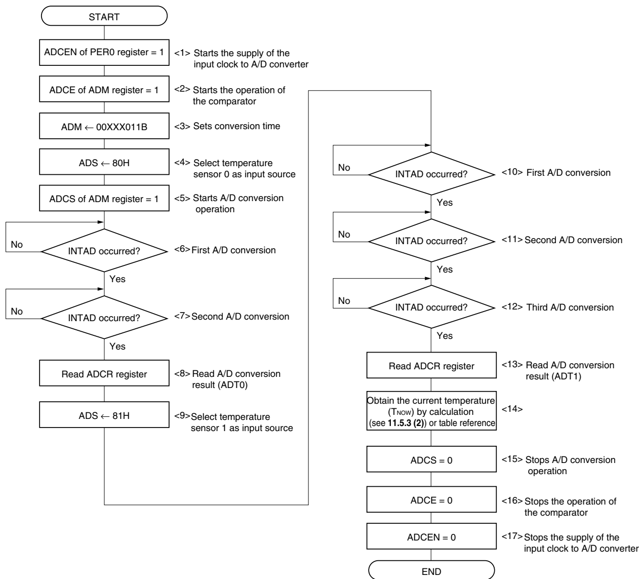
Figure 11-18. Flowchart of Procedure for Using Temperature Sensor
