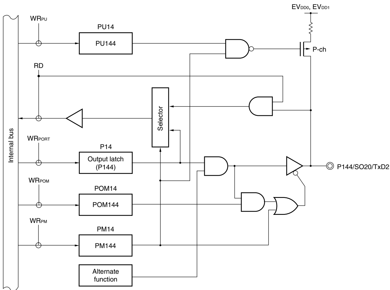
Figure 4-38. Block Diagram of P14
