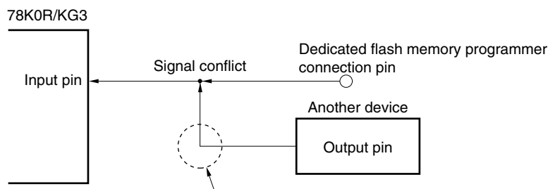
Figure 25-6. Signal Conflict ( \overline{\text{RESET}} Pin)
