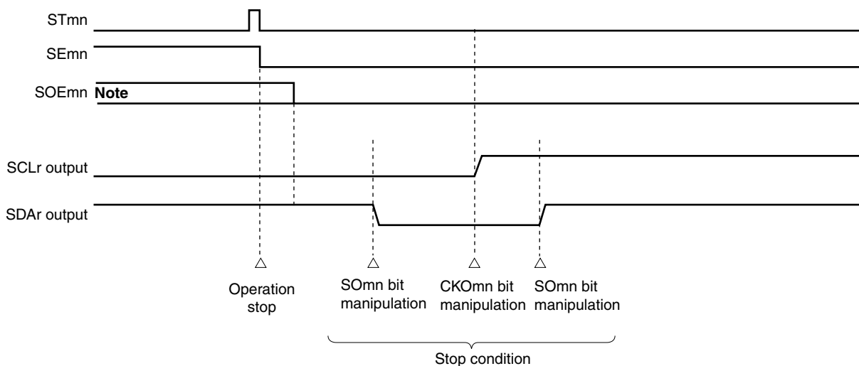
Figure 13-103. Timing Chart of Stop Condition Generation
