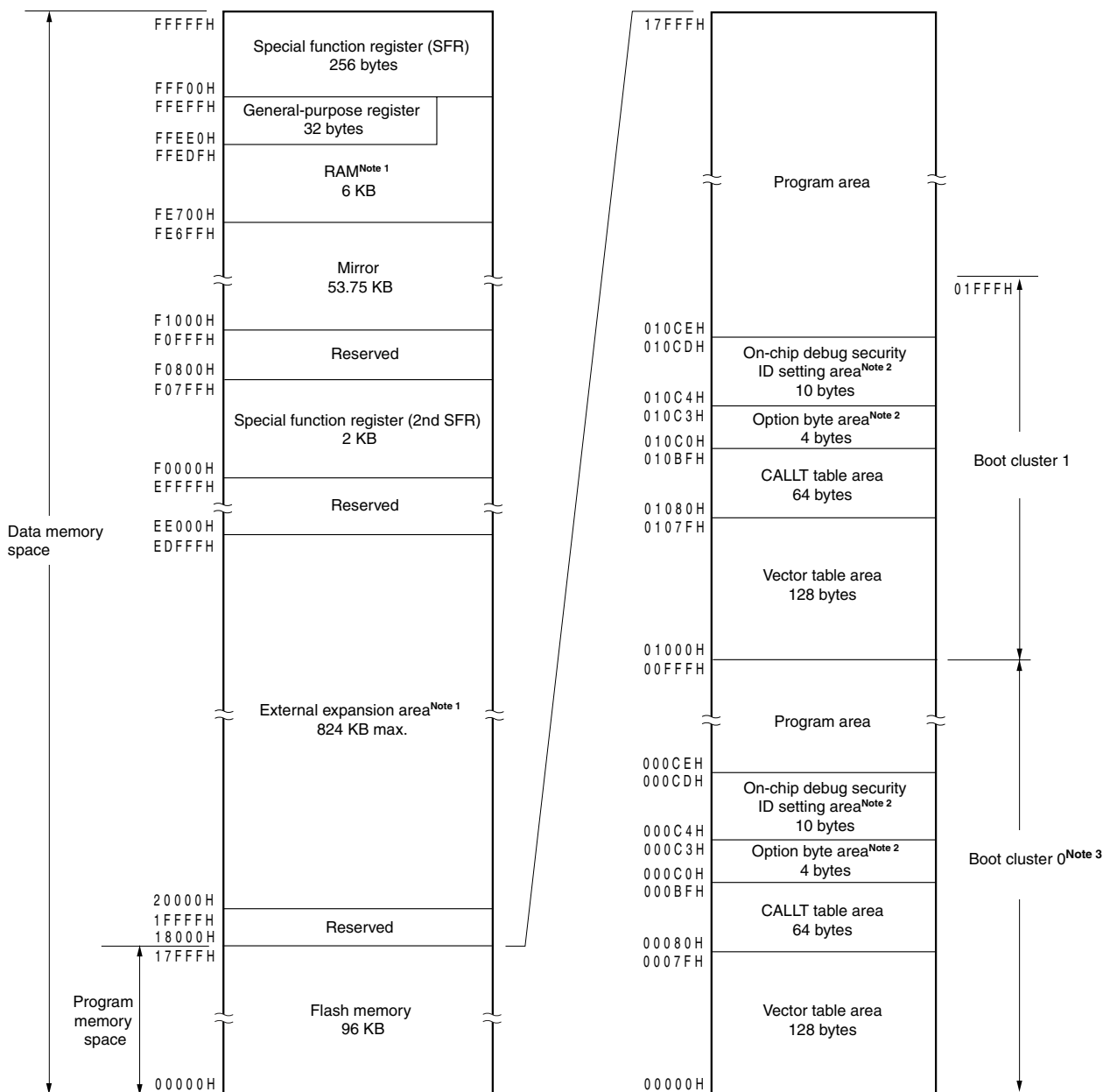
Figure 3-2. Memory Map ( \mu PD78F1163, 78F1163A)
