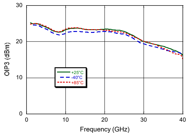
Output IP3
