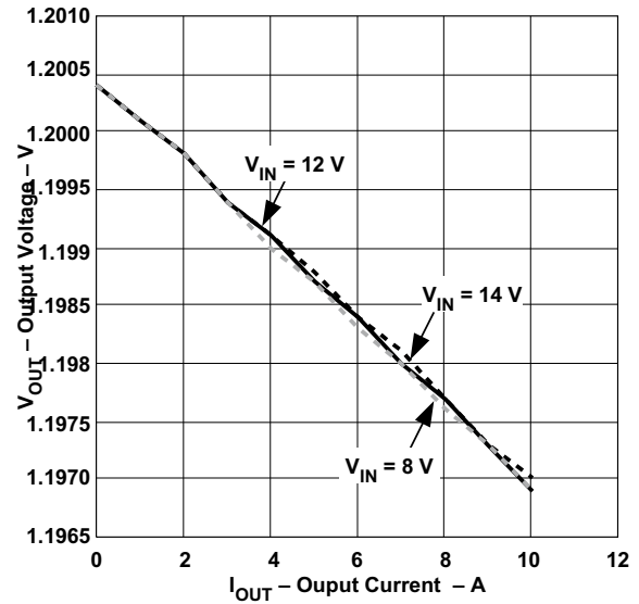
Figure 9-2. Load Regulation
