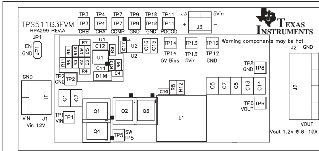
Figure 10-1. Top Layer Assembly Drawing (Top View)
