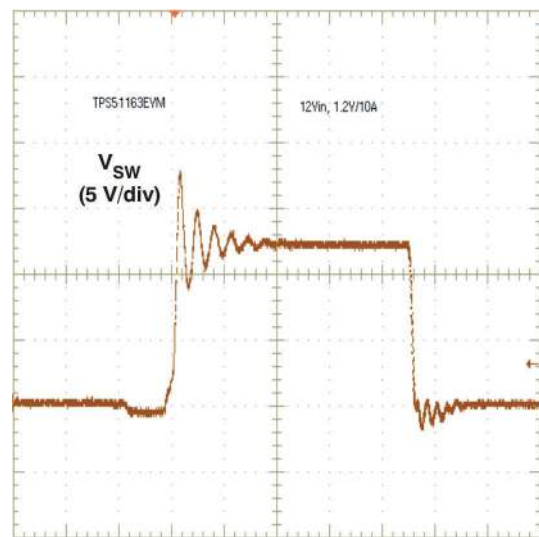
t - Time - 40 ns/div Figure 9-8. Switch Node Waveform
