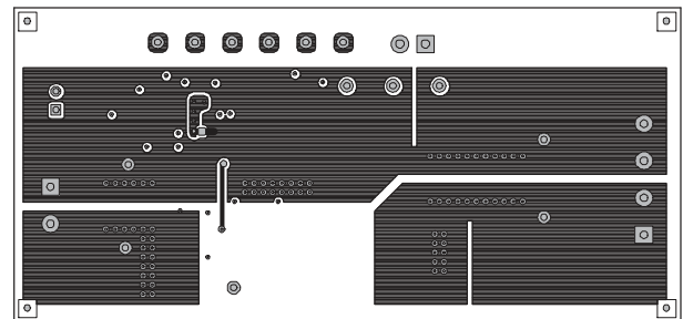
Figure 10-6. Bottom Copper (Top View)
