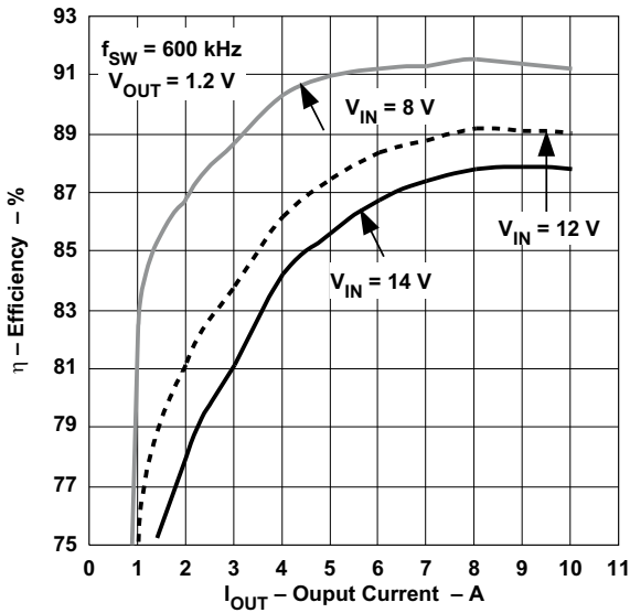
Figure 9-1. Efficiency
