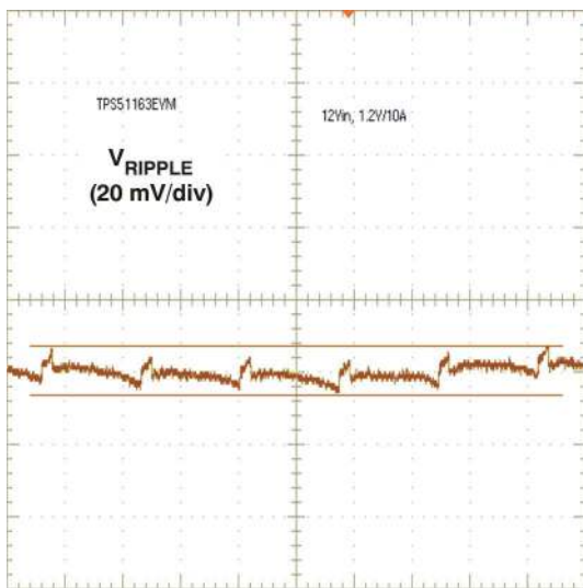
t - Time - 1 \mu s/div Figure 9-7. Output Ripple
