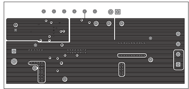
Figure 10-4. Internal Layer 1
