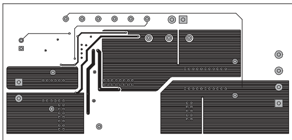
Figure 10-5. Internal Layer 2
