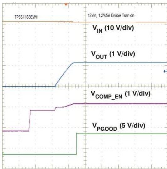
t - Time - 4 ms/div Figure 9-9. Enable Turn-On
