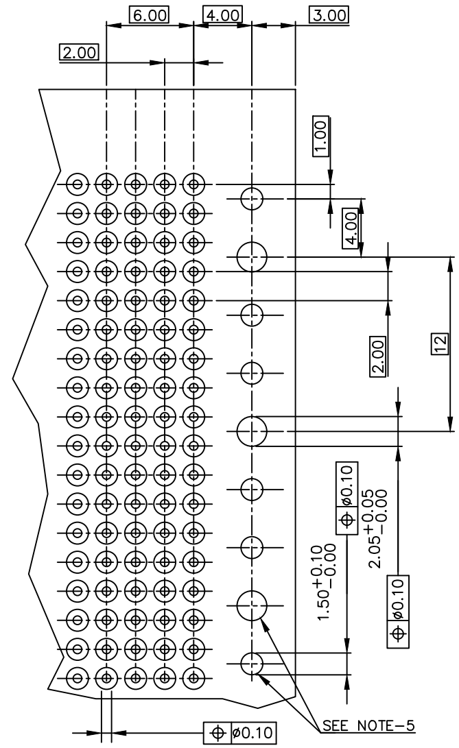
RECOMMENDED PC BOARD LAYOUT, COMPONENT SIDE. FOR PTH DIMENSIONS REFER DRAWING NO : 58351.
