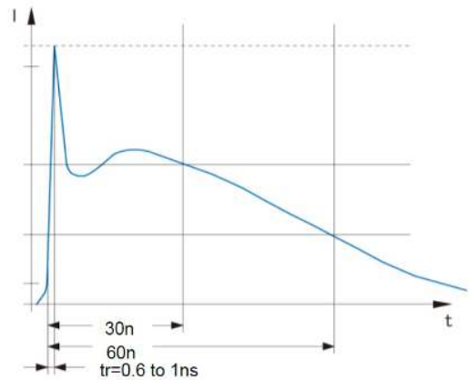
IEC61000-4-2 Waveform
