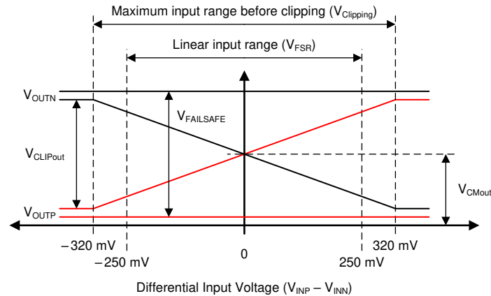
Figure 7-2. Output Behavior of the AMC1301
