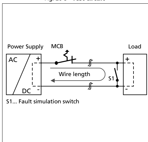
Fig. 26-5 Test circuit
