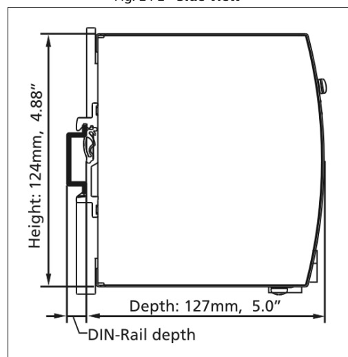
Fig. 24-2 Side view
