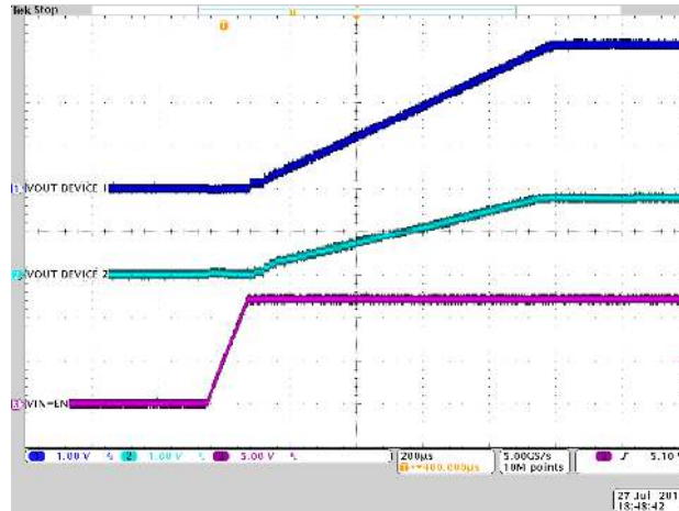
Figure 10-83. Tracking
