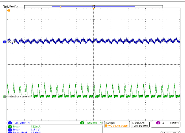
Vin = 5 V PFM Io = 0.1 A Vout = 1.8 V FSEL = high TA = 25 °C
