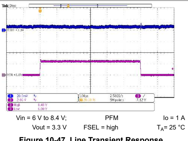
Figure 10-47. Line Transient Response
