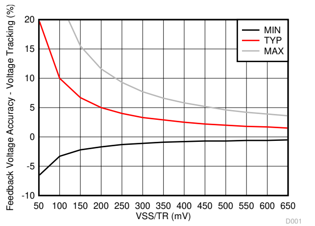
Figure 10-79. Feedback Voltage Accuracy with Voltage Tracking vs Voltage at VSS/TR
