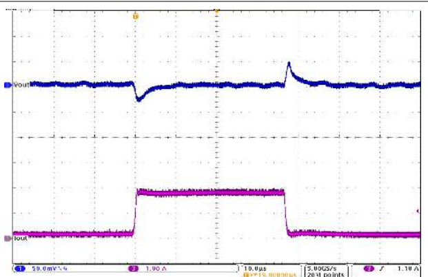
Vin = 12 V PWM Io = 200 mA to 1.8 A Vout = 1.8 V FSEL = high TA = 25 °C
