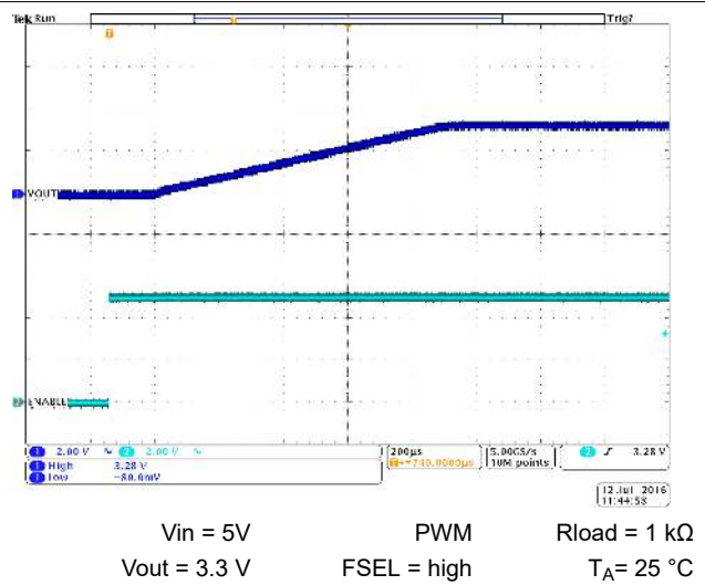
Figure 10-49. Start-Up Timing
