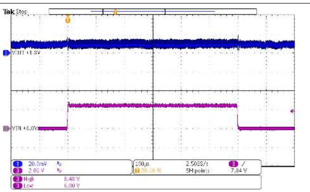
Vin = 6 V to 8.4 V; PWM Io = 1 A Vout = 1.8 V FSEL = high TA = 25 °C
