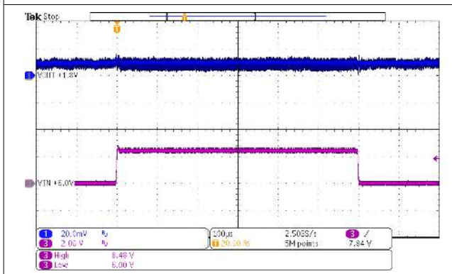
Vin = 6 V to 8.4 V; PFM Io = 1 A Vout = 1.8 V FSEL = high TA = 25 °C
