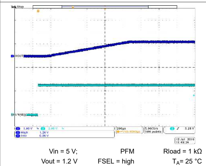
Figure 10-35. Start-Up Timing
