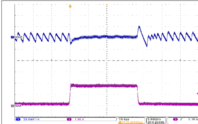
Vin = 12 V PFM Io = 200 mA to 1.8 A Vout = 1.8 V FSEL = high TA = 25 °C
