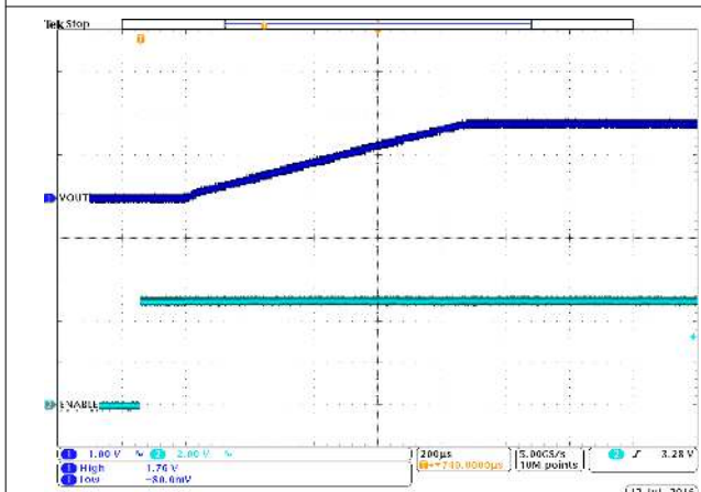
Vin = 5 V PWM Rload = 1 kΩ Vout = 1.8 V FSEL = high TA = 25 °C
