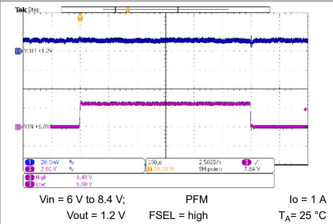
Figure 10-33. Line Transient Response
