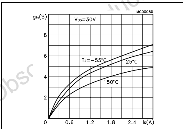
Figure 17. Transconductance p-ch
