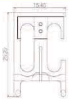
Dimensions - mm
