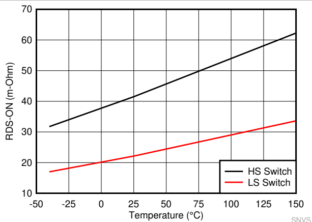
Figure 7-5. High-Side and Low-Side Switches R_{DS\_ON}
