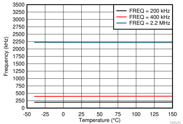
Figure 7-4. Switching Frequency
