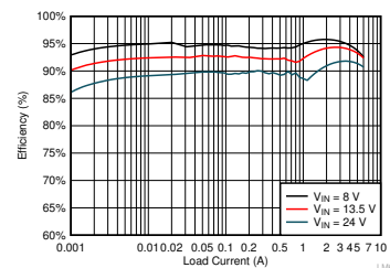
Efficiency: V_{\text{OUT}} = 5\text{ V} , F_{\text{SW}} = 2.1\text{ MHz}
