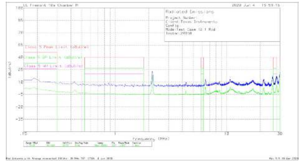
V_{OUT} = 5\text{ V} F_{SW} = 2.1\text{ MHz} I_{OUT} = 4\text{ A} Frequency Tested: 150 kHz to 30 MHz
