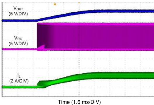
Figure 9-19. LMQ62440-Q1 Start-up with 3.25-A
