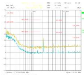
Conducted EMI: V_{\text{OUT}} = 5\text{ V} , I_{\text{OUT}} = 4\text{ A}
