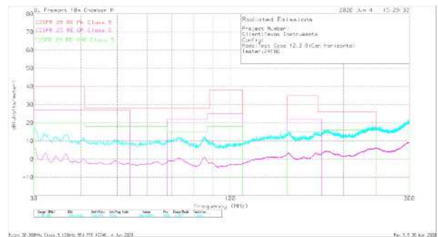
V_{OUT} = 5\text{ V} F_{SW} = 2.1\text{ MHz} I_{OUT} = 4\text{ A} Frequency Tested: 30 MHz to 300 MHz
