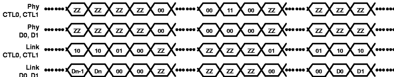
Figure 6. Transmit Timing
