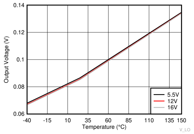
A. I_O=100\text{mA} Figure 6-18. LO Low Output Voltage ( V_{LOL} )
