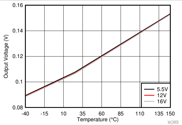
A. I_O=100\text{mA} Figure 6-20. HO Low Output Voltage ( V_{HOL} )
