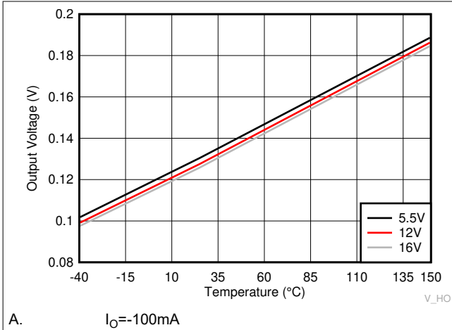
Figure 6-21. HO High Output Voltage ( V_{HOH} )
