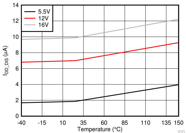
A. V_{EN} = 0\text{ V} Figure 6-5. VDD Current When Disabled
