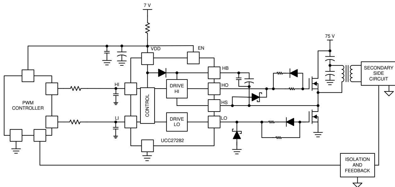
Figure 8-1. Typical Application
