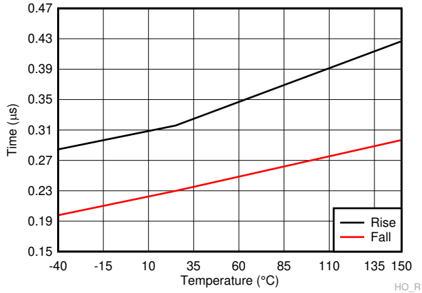
A. C_L=100nF Figure 6-27. HO Rise & Fall Time
