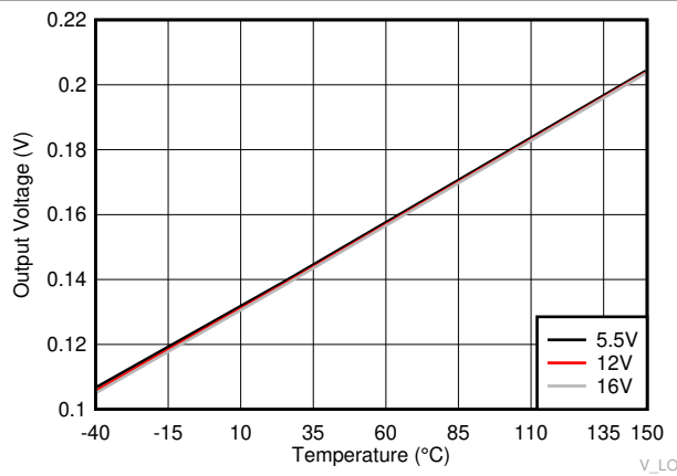
A. I_O=-100\text{mA} Figure 6-19. LO High Output Voltage ( V_{LOH} )
