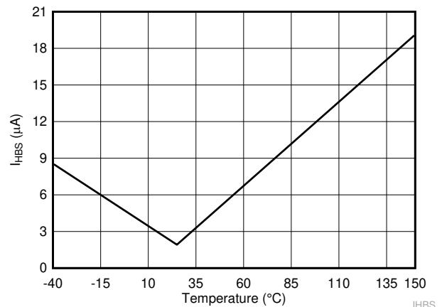
A. V_{HB} = V_{HS} = 100\text{ V} Figure 6-6. HB to VSS Quiescent Current
