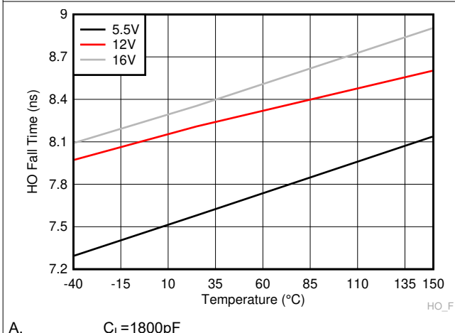
Figure 6-25. HO Fall Time
