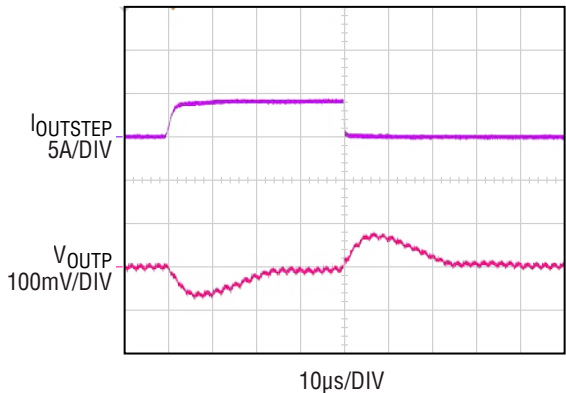
Figure 3. Load Transient (4A to 8A) Response Waveform at 12V IN and 1.5V out , 10 \mu s/div
