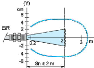
(Y) \varnothing of beam With reflector XU5C50
