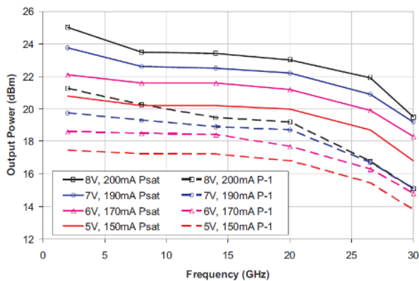
Output Power
