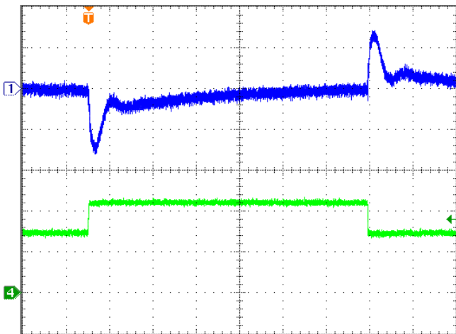
Fig.3.3V-6: Output voltage response to load current step-change (10A \leftrightarrow 15A) at Vin=48V. Top trace: Output voltage (100mV/div). Bottom trace: load current (5A/div). Current slew rate: 5A/us. Co=470uF os-con + 10uF tantalum + 1uF ceramic. Time scale: 100us/div
