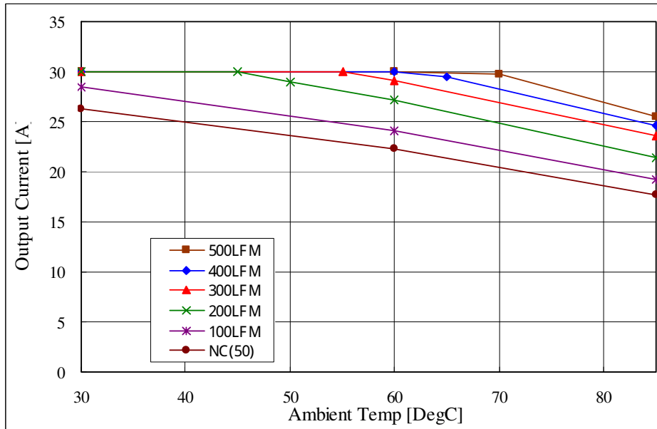
Fig.3.3V-1: Available load current vs. ambient temperature and airflow rates for Vin=48V. Maximum component temperature \leq 125^{\circ}\text{C}
