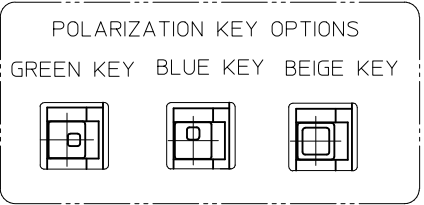
DETAIL C
