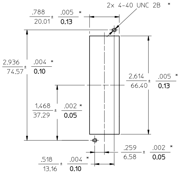
VIEW A RECOMMENDED MOUNTING HOLES SCALE: 1:1
