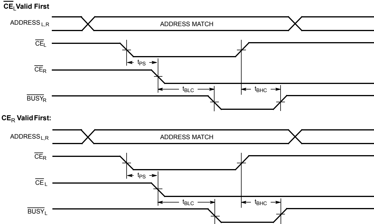
Figure 14. Busy Timing Diagram No.1 ( \overline{CE} Arbitration) [47]
