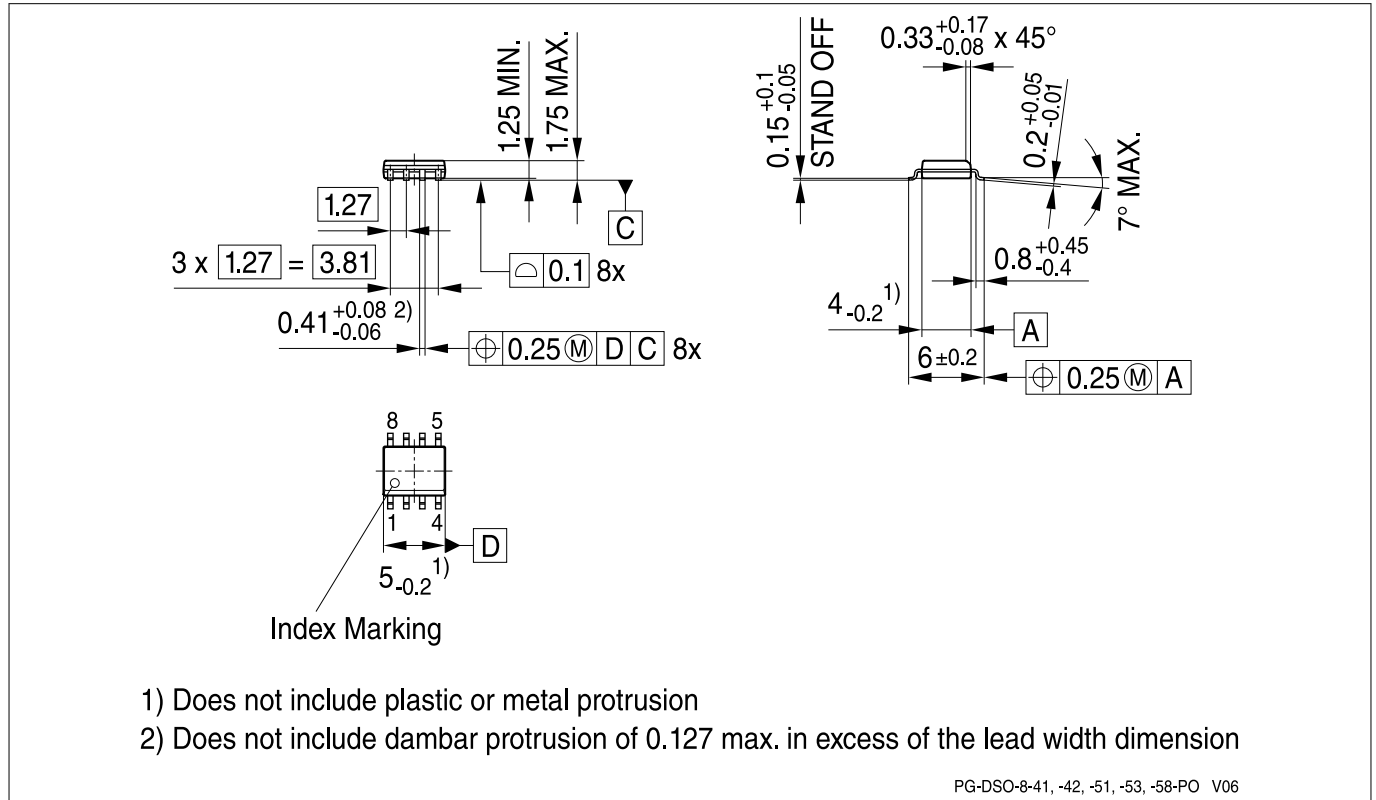
Figure 18 Package Dimensions for PG-DSO-8
