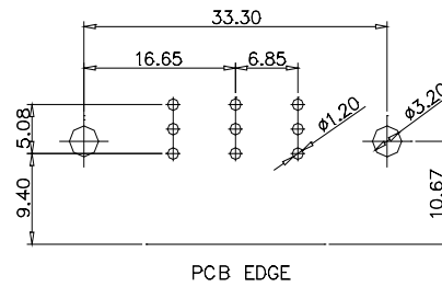
CODE:3W3/3WK3 MALE/FEMALE
