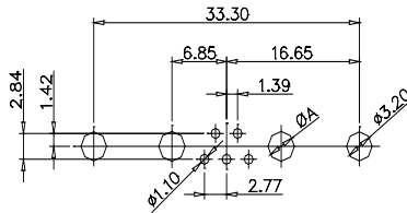
CODE:11W1 MALE/FEMALE
