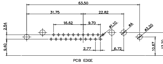
CODE:36W4 FEMALE
