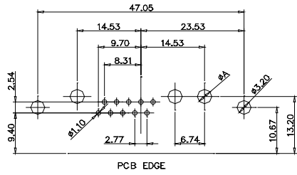
CODE:13W3 FEMALE
