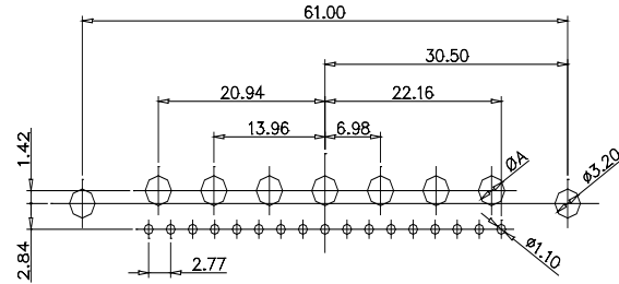
CODE:21W4 MALE/FEMALE
