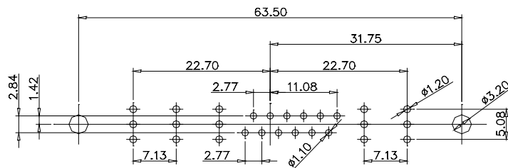
CODE:17W5 FEMALE
