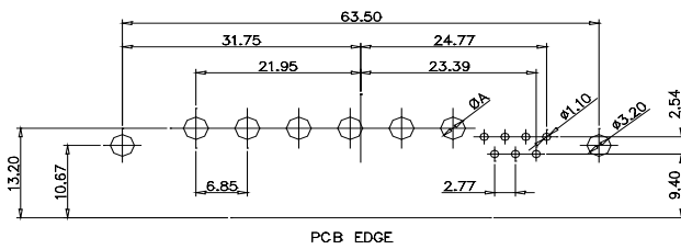
CODE:13W6 MALE
