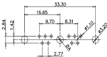
CODE:17W2 MALE/FEMALE
