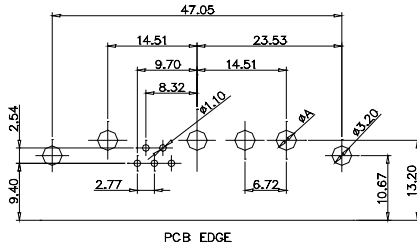
CODE:9W4 FEMALE
