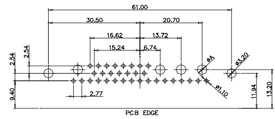
CODE:36W4 FEMALE
