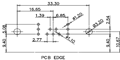
CODE:11W1 MALE/FEMALE
