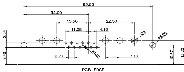
CODE:17W5 MALE
