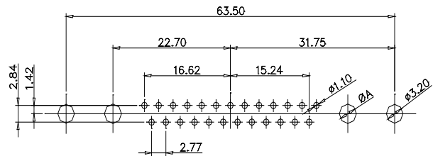
CODE:21W1 MALE/FEMALE
