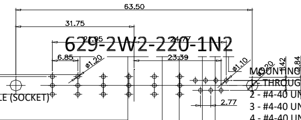
CODE:13W6 MALE
