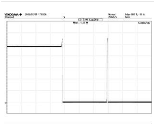
Figure 7: Output over voltage protection at 110/220Vac, 12.5A Iout. VOUT: 5V/div, 500mS/div
