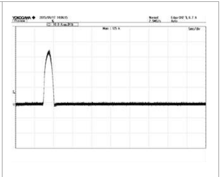
Figure 8: Inrush current @ Vin=220Vac. Iin: 10A/div, 5mS/div;
