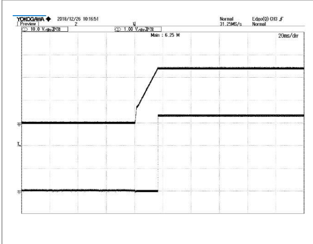
Figure 9: PG voltage vs. Vout @ Vin=220Vac, 0A Iout TOP: Vout, 10V/div, 20mS/div BOTTOM: PG, 1V/div, 20mS/div
