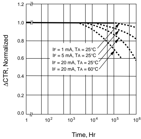
CTR DEGRADATION
