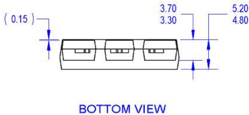
Figure 23. TO264, Molded, 3-Lead, Jedec Variation AA
