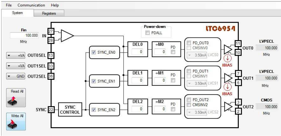
Figure 5. LTC6954-2 Settings
