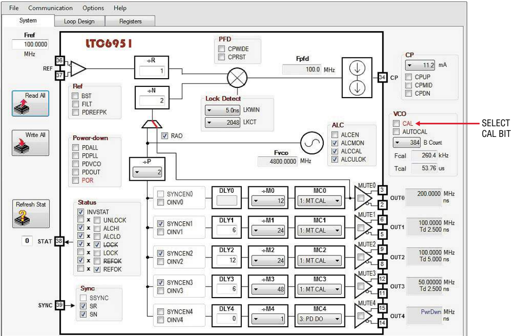
Figure 4. LTC6951 Settings
