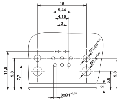
Drilling diagram
