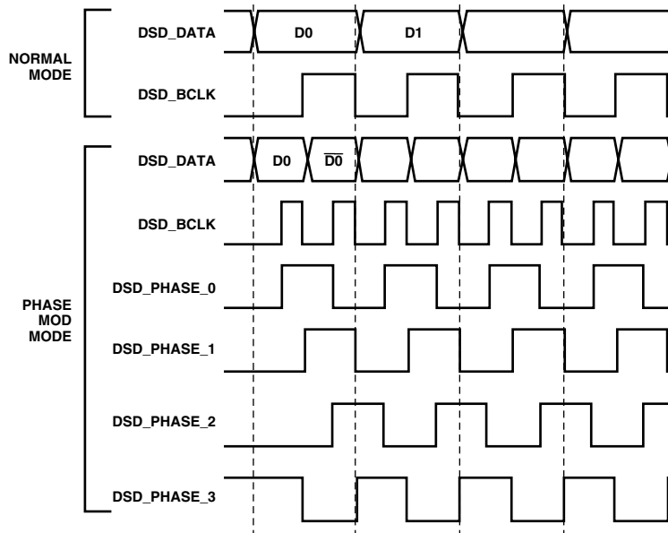
Figure 3. DSD Modes
