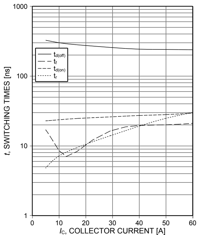
Figure 8. Typical switching times as a function of collector current (inductive load, T_{vj}=175^\circ\text{C} , V_{CE}=400\text{V} , V_{GE}=0/15\text{V} , R_{Gon}=13\Omega , R_{Goff}=13\Omega , dynamic test circuit in Figure E)
