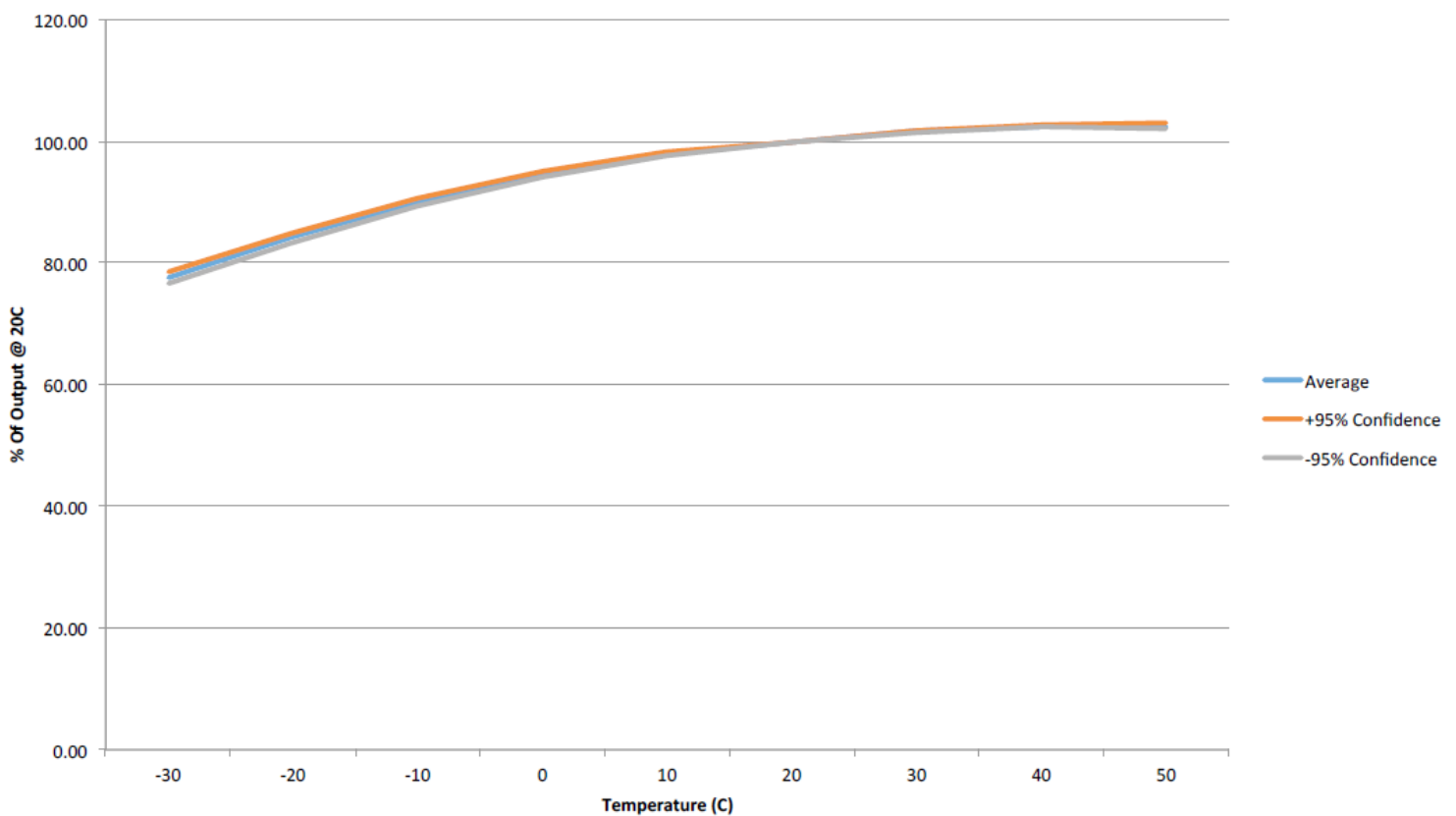
Output vs Temp
