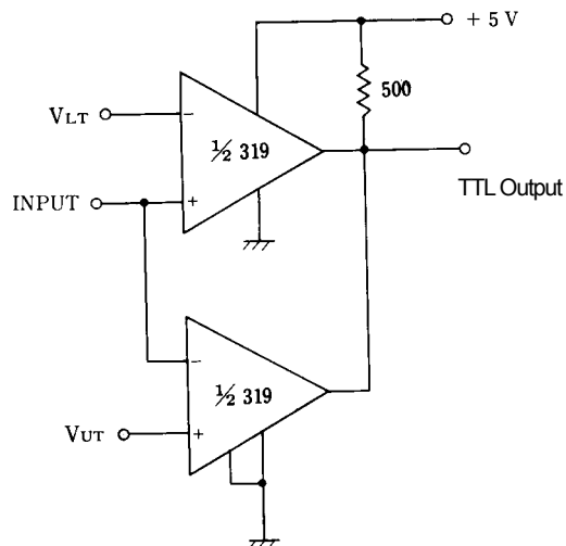
Window Detector
