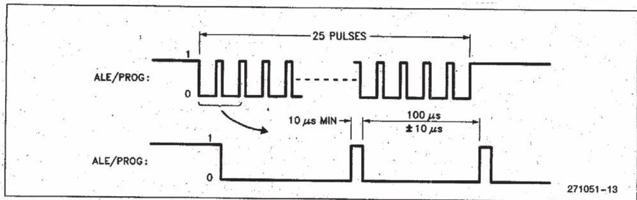
Figure 10. \overline{\text{PROG}} Waveforms
