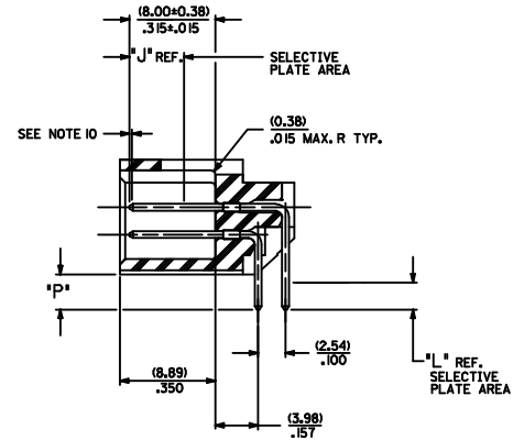
SECTION J-J
