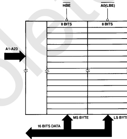
FIGURE 3-28. Memory Interface
