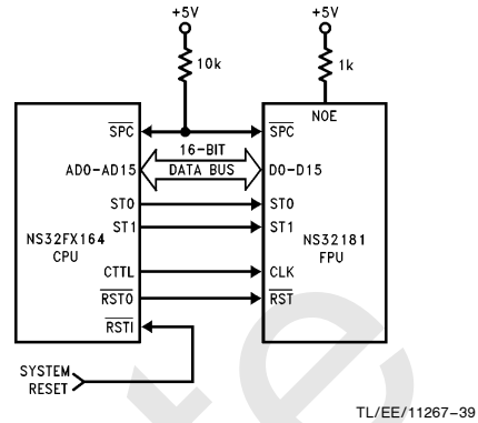
FIGURE 3-27. NS32FX164 and FPU Interconnections
