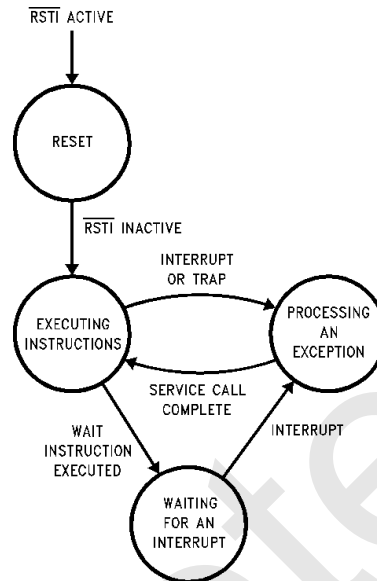
FIGURE 3-1. Operating States
