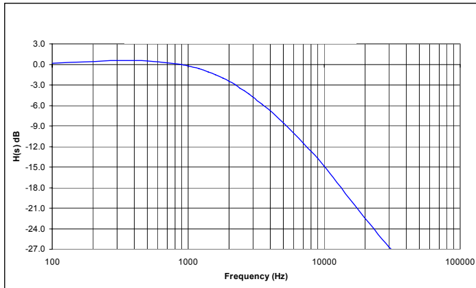
Figure 8 Jitter Transfer Characteristic - ACS8947T Stand-alone
