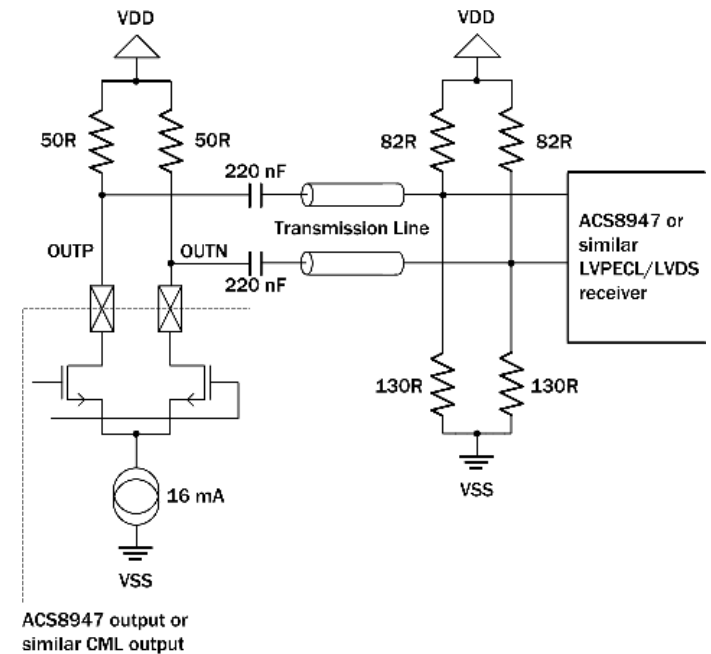
Figure 15 Generic CML Output AC Coupled to LVPECL Receiver
