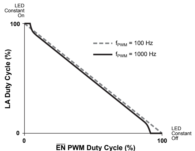
Figure 11: LA Duty Cycle vs. \overline{EN} PWM Duty Cycle
