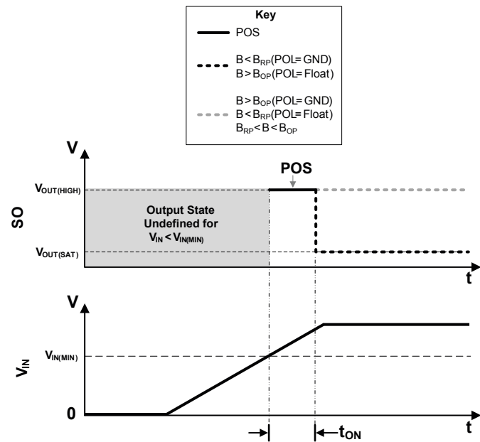
Figure 5: Power-On Timing
