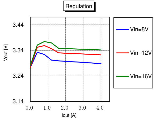
Vout vs. Line Voltage and Load Current @ +25° C. (Vout = 3.3V)
