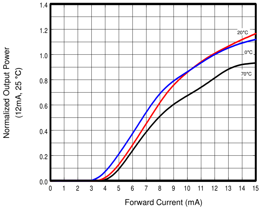
Output Power vs. Forward Current
