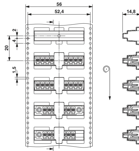
Dimensioned drawing
