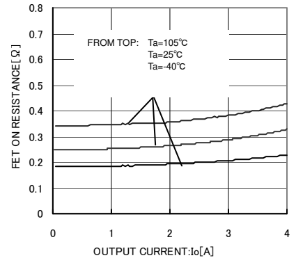
Fig.21 ON Resistance VIN=13.2V (BD9009HFP)
