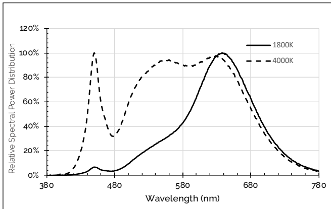
Figure 24: 1800K - 4000K with 90 CRI
