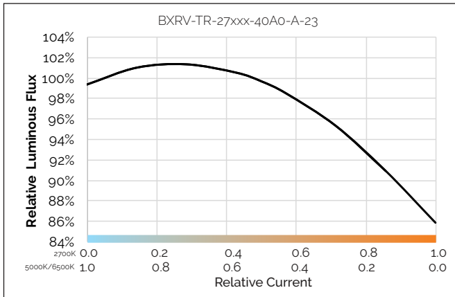
Figure 16: Relative Flux vs. Relative Current
