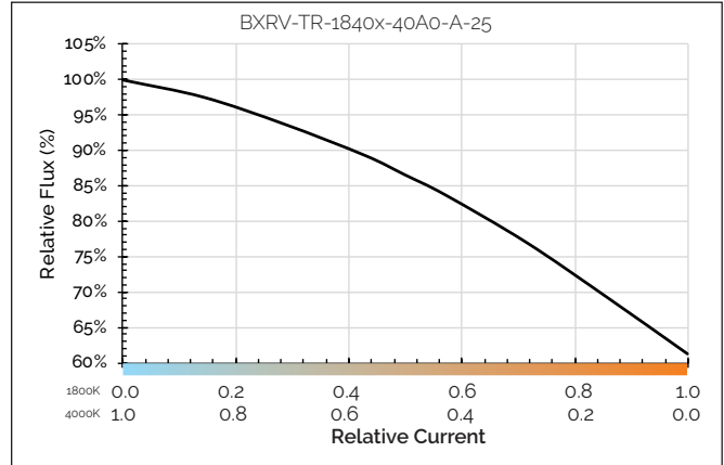
Figure 17: Relative Flux vs. Relative Current
