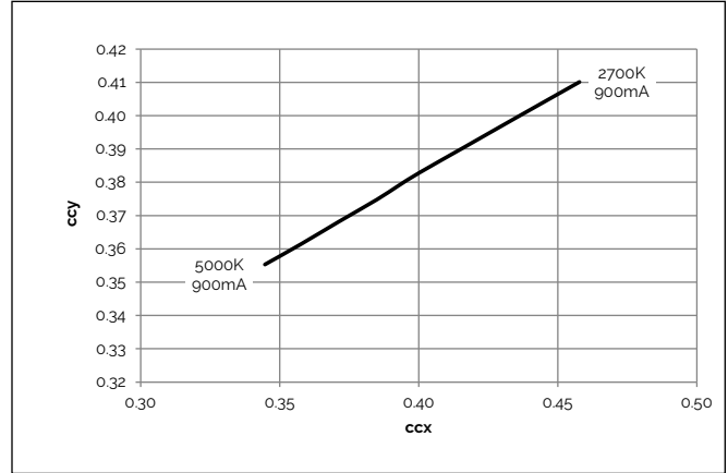
Figure 13: CCT Tuning Range, T_c = 85^\circ\text{C}
