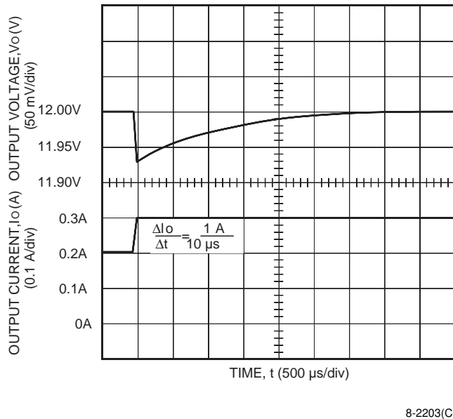
Figure 26. ME005B Typical Output Voltage Waveform for a Step Load Change from 50% to 75% of I_{o, \text{max}} with V_i = 48 \text{ V} and T_A = 25 \text{ }^\circ\text{C}
