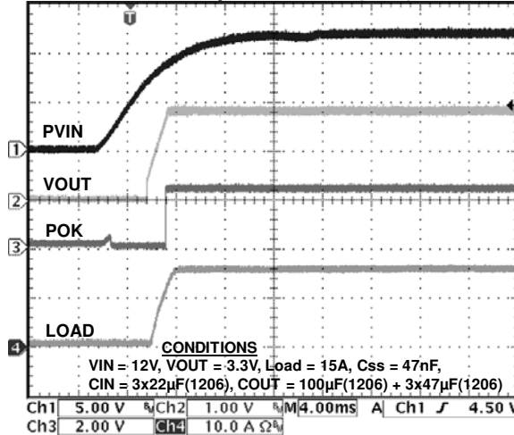
Power Up Waveform (15A)
