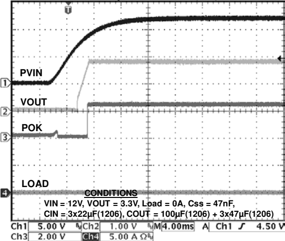
Power Up Waveform (0A)
