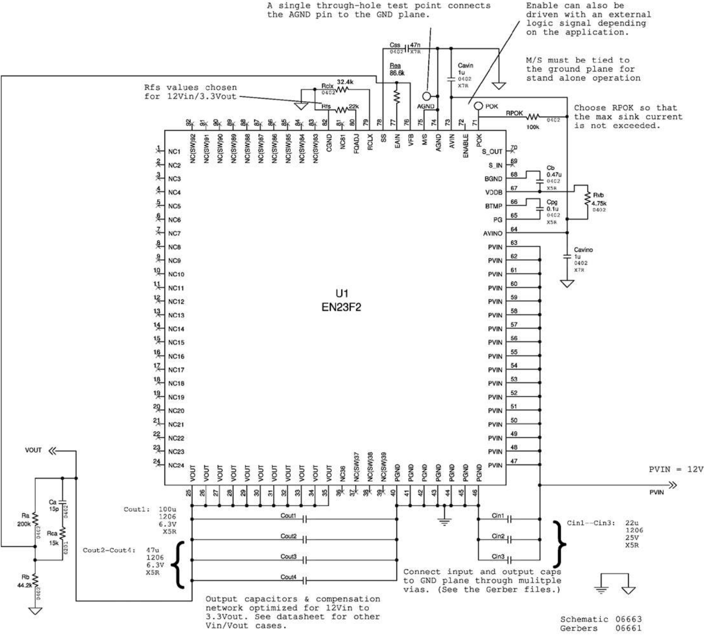
Figure 13: Engineering Schematic
