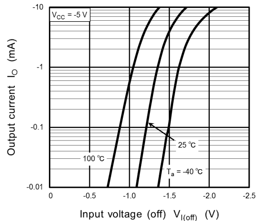
Fig. 7.2 I_O - V_{I(off)}
